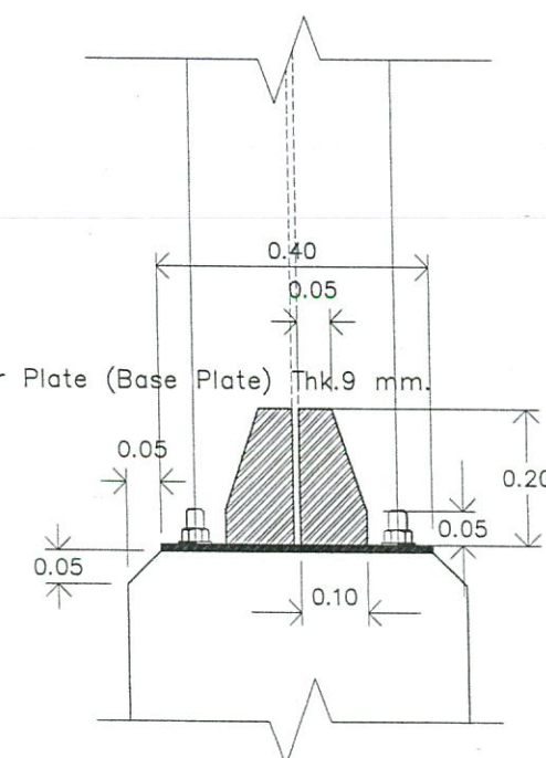
SIDE VIEW DETAIL SCALE NOT TO SCALE
