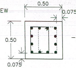
SECTION A - A SCALE 1 : 25
