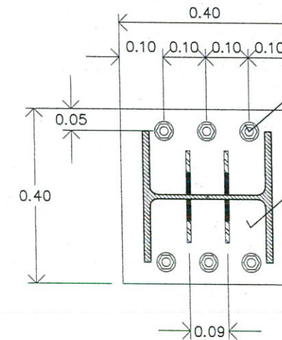
BASE PLATE DETAIL SCALE NOT TO SCALE
